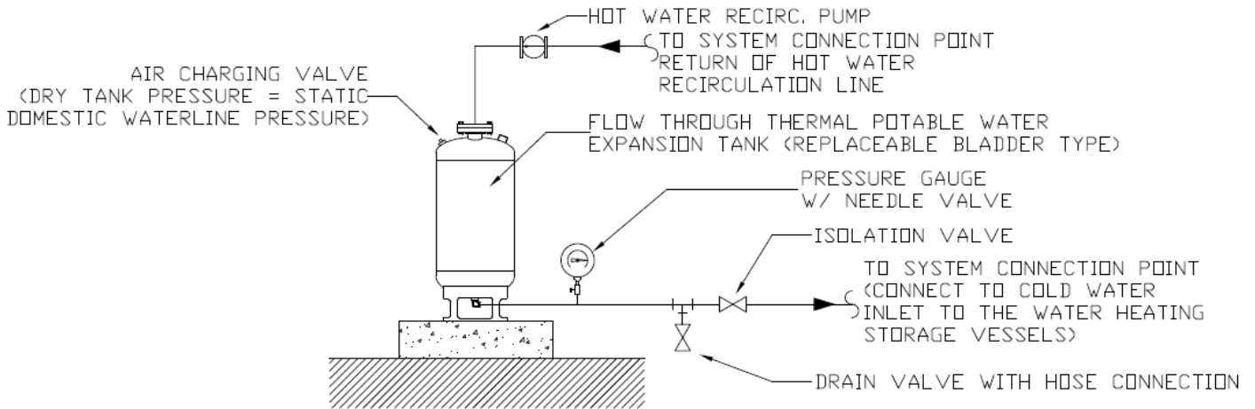
THERMAL EXPANSION TANK DETAIL - FORCED CIRCULATION - HIGH TEMP NOT TO SCALE
